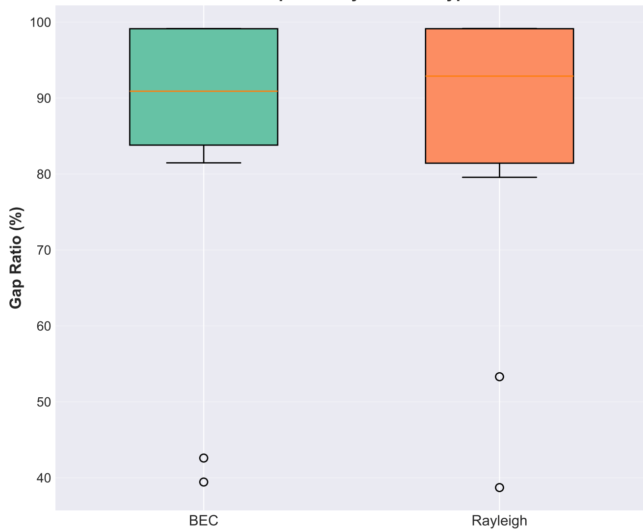
CE Gap Ratio by Channel Type
