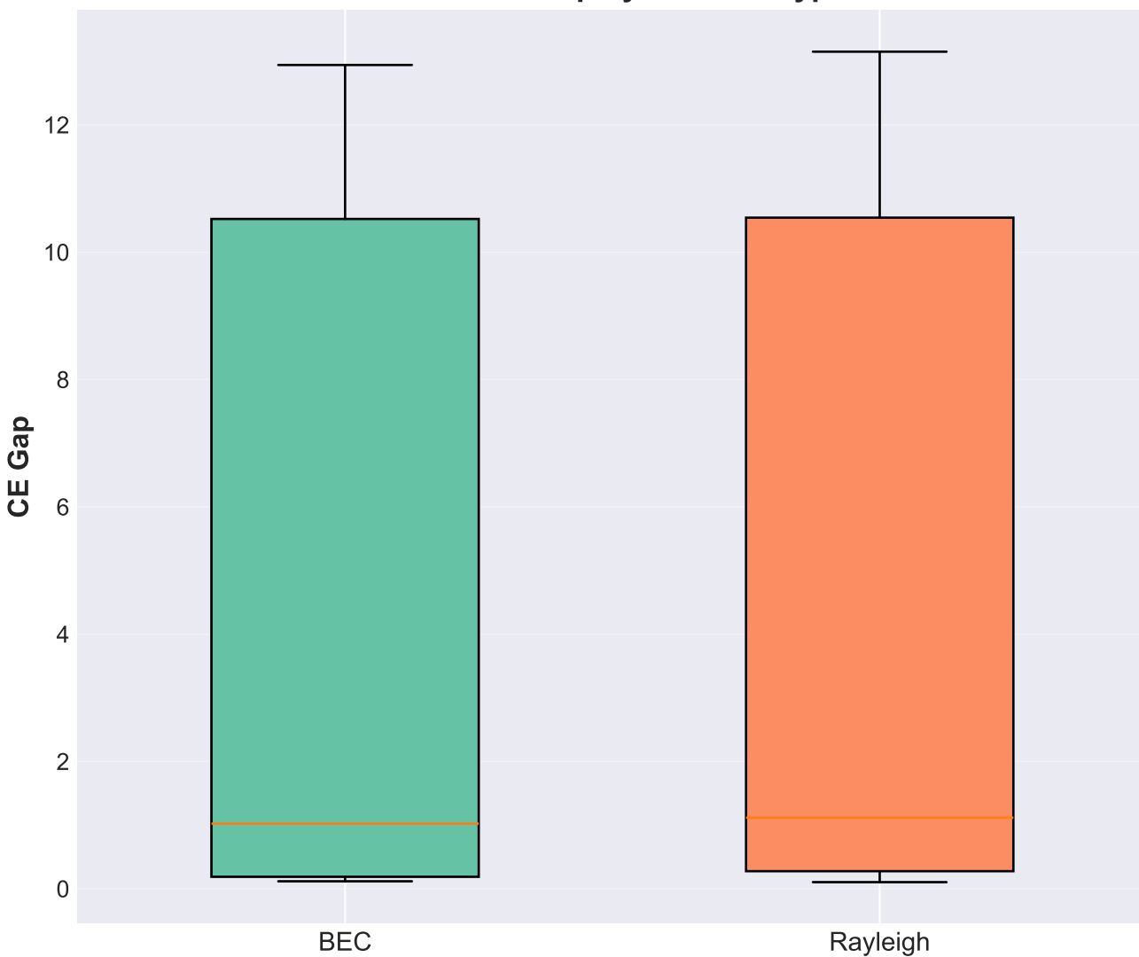
CE Gap Ratio by Channel Type
