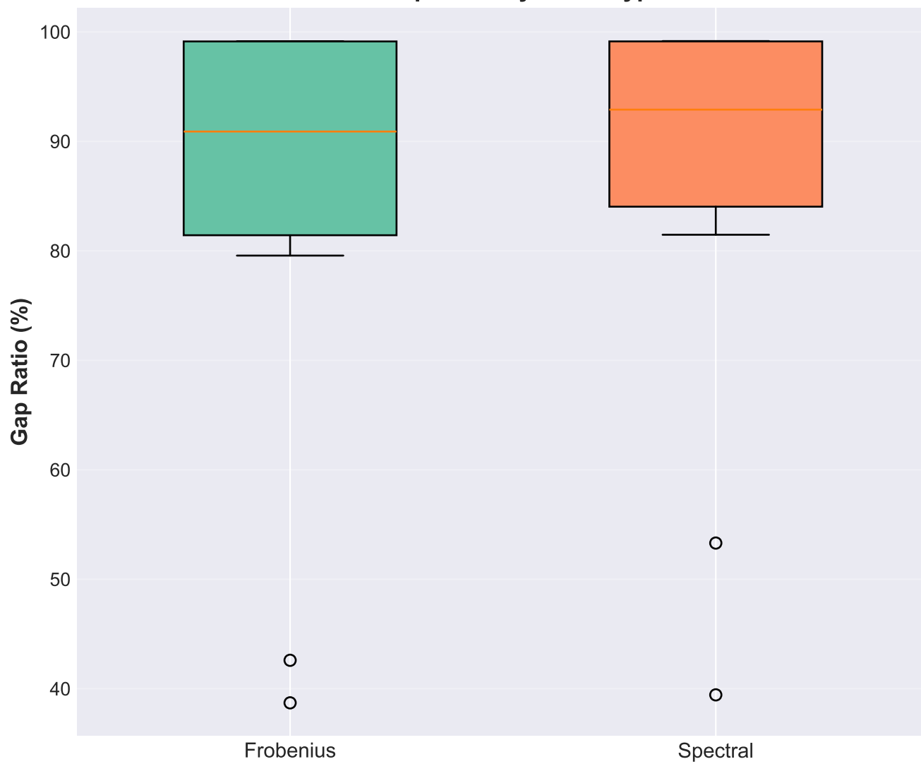
CE Gap Ratio by Norm Type
