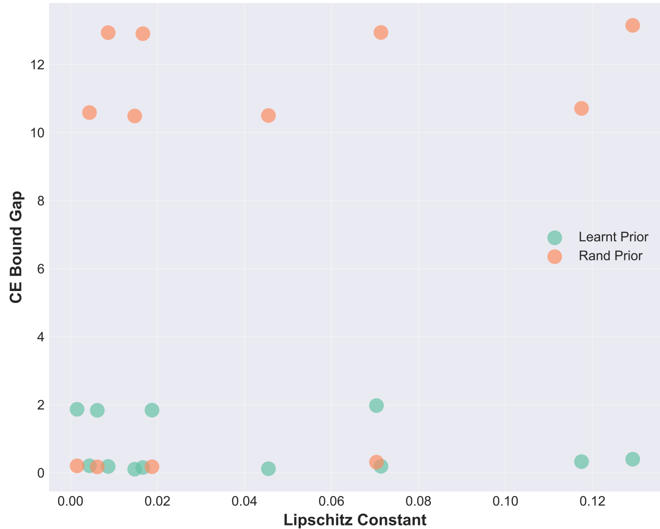
Impact of Lipschitz Constant on Bound Gap
