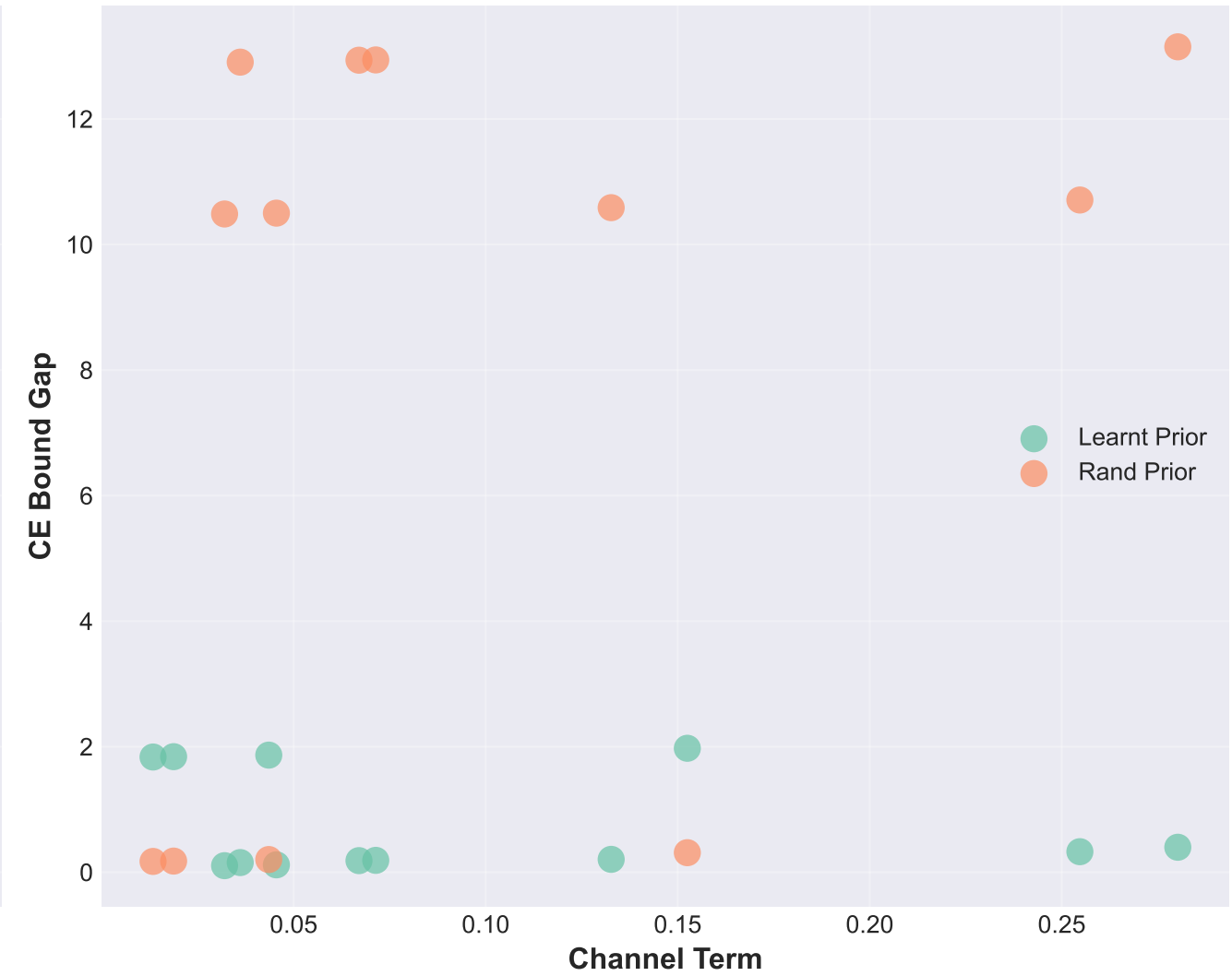
Impact of Channel Term on Bound Gap
