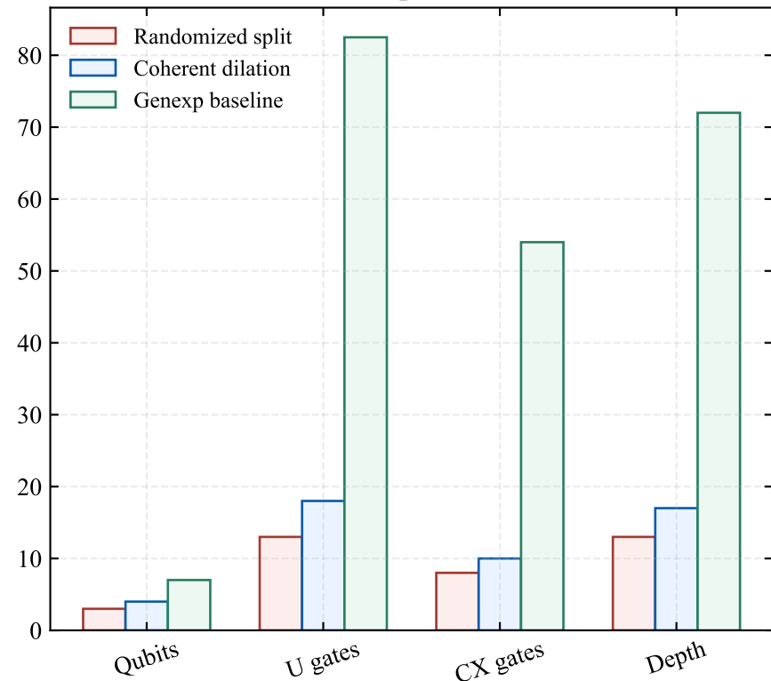
Per-shot compiled resources
