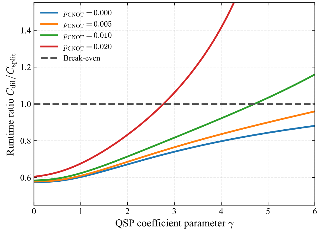
QSP Jordan family under noise
