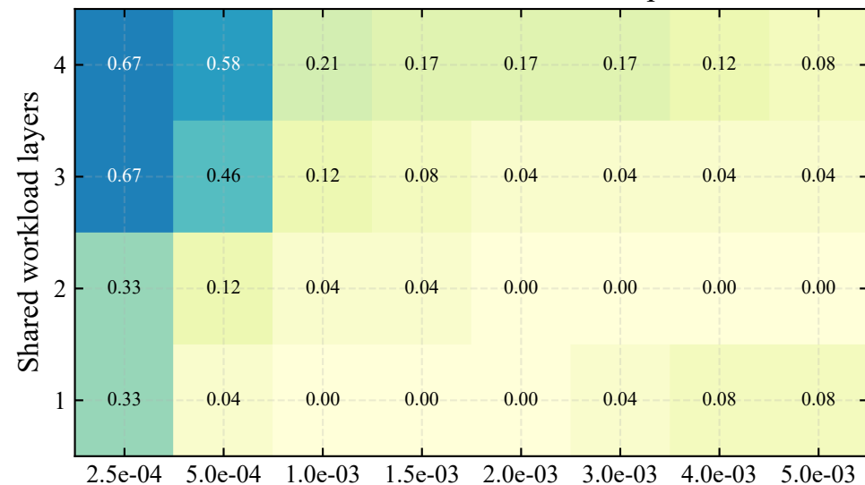
Beneficial fraction: dilation / split
