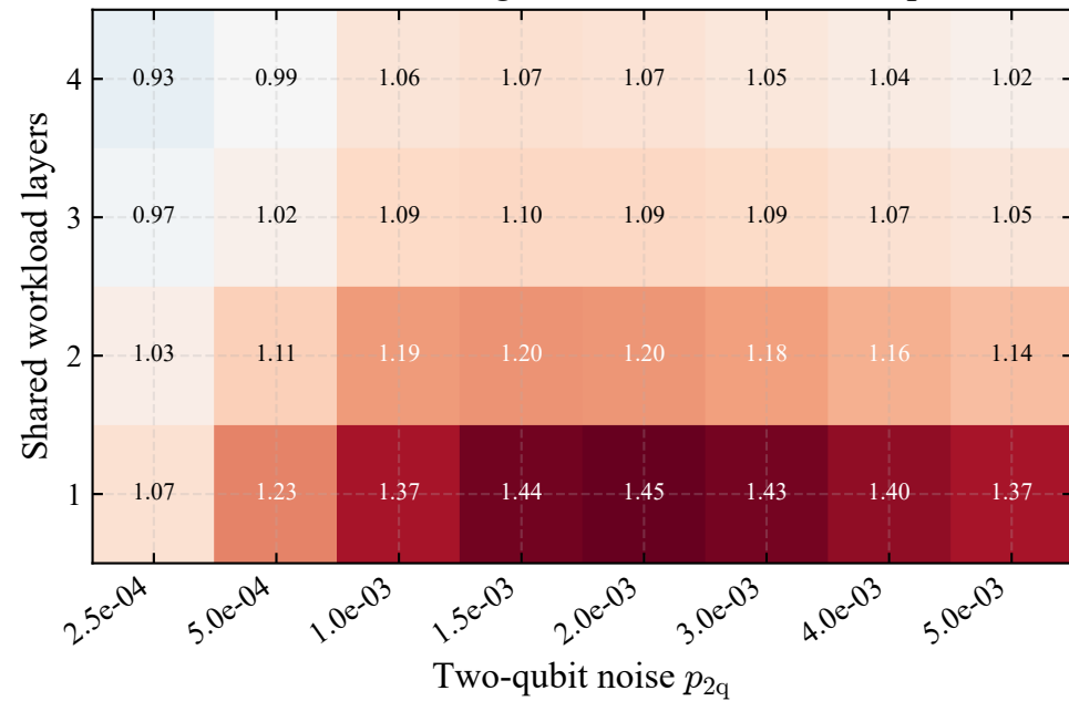
Median finite-budget MSE ratio: dilation / split
