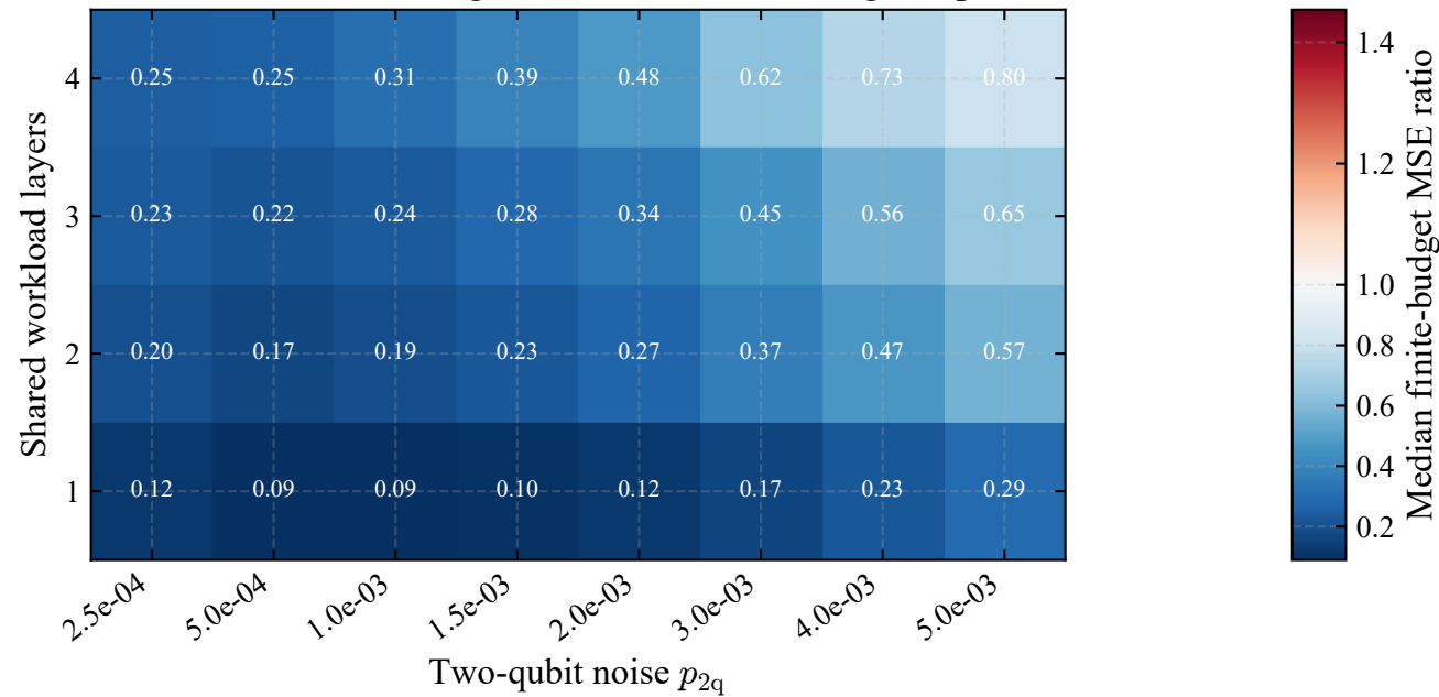
Median finite-budget MSE ratio: dilation / genexp
