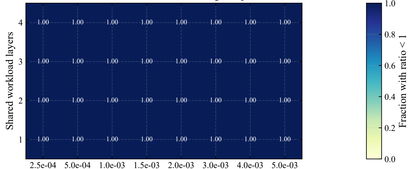
Beneficial fraction: dilation / genexp
