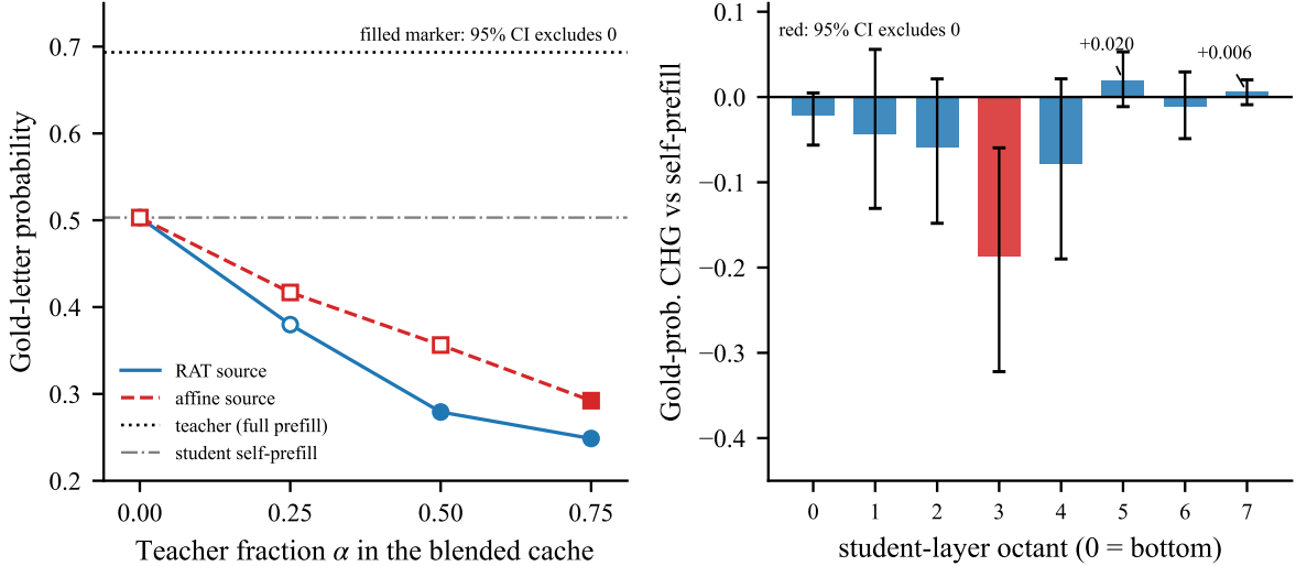
Figure 3: Oracle probes on Qwen3-4B→1.7B ( n=30 ; the fraction probe is confirmatory, the best-source replication and the octant sweep are frozen-gate extensions, Section 3.3). Left: gold-letter probability as translated teacher content replaces the student’s own cache, for two content sources. Filled markers mark mixture fractions whose paired CHG interval excludes zero: the decline separates from the student from \alpha=0.5 onward for the RAT source and only at \alpha=0.75 for the affine source, and no mixture at either source yields a gain whose interval excludes zero. Right: window injection per student-layer octant (affine source), plotted as gold-probability CHG with 95% CIs. Only the octant spanning layers 10–13 excludes zero; two top-layer octants carry small positive point estimates whose intervals span zero.
