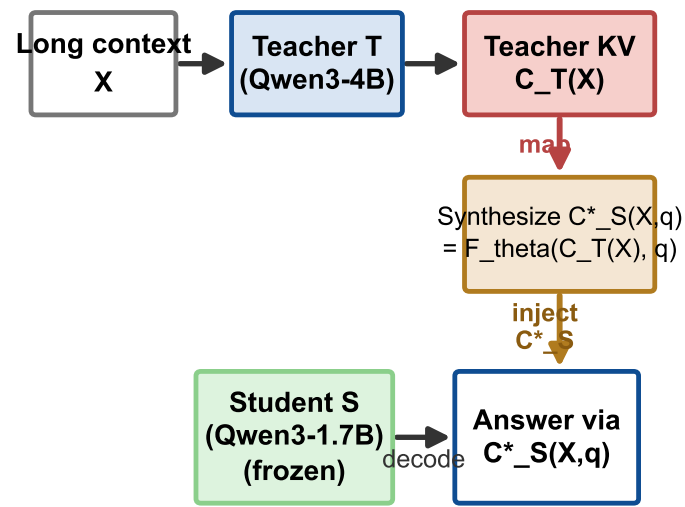
(a) Scenario: synthesize then hand off KV state
