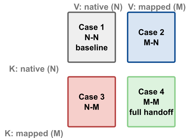
(b) Four diagnostic arms (native vs. mapped K/V)
