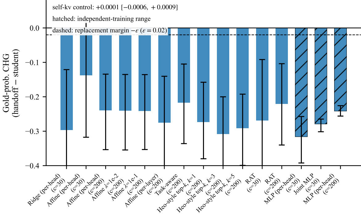
Figure 2: The translator landscape on the primary pair: gold-letter-probability change over the student’s own prefill with 95% bootstrap intervals, one bar per configuration. All point estimates are negative; the best of them (per-head affine at c=30 ) is the only one whose interval reaches zero. Across the calibration ladder the affine estimate moves by 0.02 in total (Table 1), and the architecture-anchored, gradient-trained, and over-parameterized translators all sit inside the same band. The long-sequence concatenation variants of the closest published design are reported in Table 1 and omitted here for readability.
