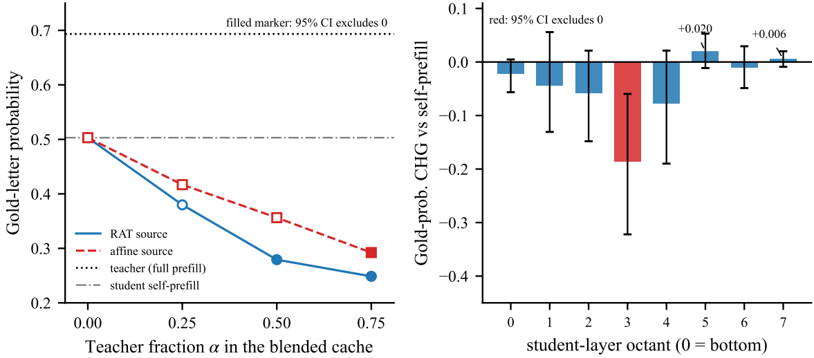
Figure 3: Oracle probes on Qwen3-4B \rightarrow 1.7B ( n=30 ; the fraction probe is confirmatory, the best-source replication and the octant sweep are frozen-gate extensions, Section 3.3). Left: gold-letter probability as translated teacher content replaces the student’s own cache, for two content sources. Filled markers mark mixture fractions whose paired CHG interval excludes zero: the decline separates from the student from \alpha=0.5 onward for the RAT source and only at \alpha=0.75 for the affine source, and no mixture at either source yields a gain whose interval excludes zero. Right: window injection per student-layer octant (affine source), plotted as gold-probability CHG with 95% CIs. Only the octant spanning layers 10–13 excludes zero; two top-layer octants carry small positive point estimates whose intervals span zero.
