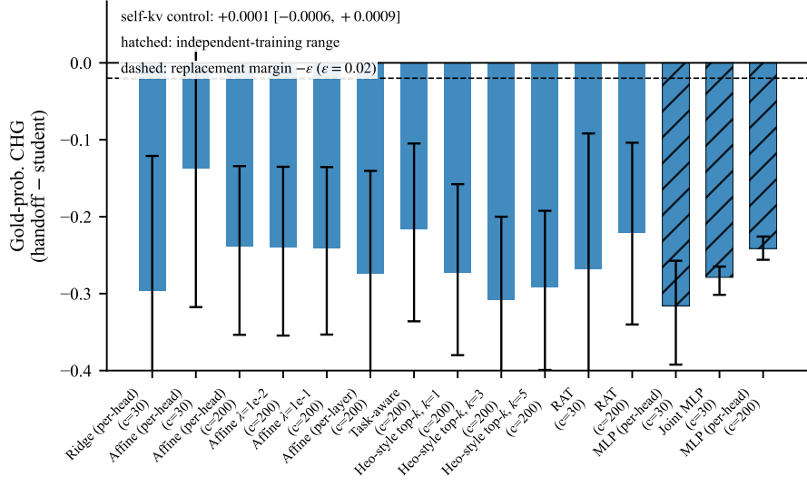
Figure 2: The mapper landscape for Qwen3-4B \rightarrow 1.7B under the unified audit protocol: gold-probability CHG over the student’s own prefill, with 95% bootstrap CIs. All primary-pair point estimates are negative and no configuration passes the replacement gate; calibration budget moves affine mapping by only 0.005 on a fixed evaluation set; the architecture-anchored RAT, the gradient-trained MLP families (hatched bars span independent trainings), and the over-parameterized joint MLP sit inside the same band. The RAT, MLP, and joint-MLP bars are frozen-gate extensions; the remaining bars are confirmatory (Section 3.3).
