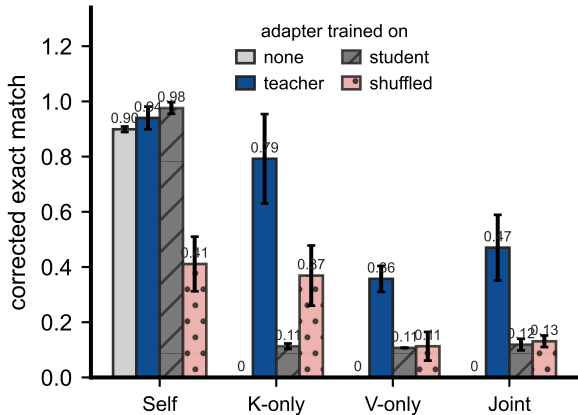
(b) 8B \rightarrow 0.6B (three seeds)
