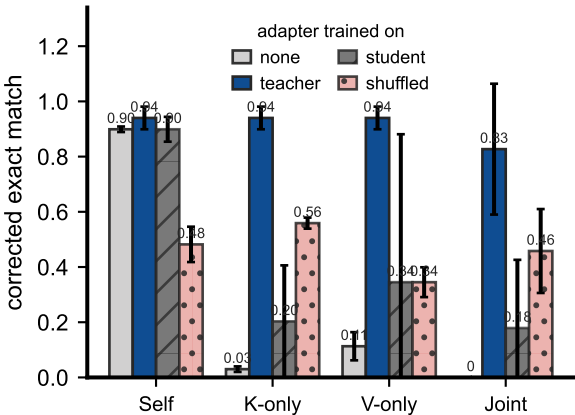
(a) 1.7B \rightarrow 0.6B (three seeds)
