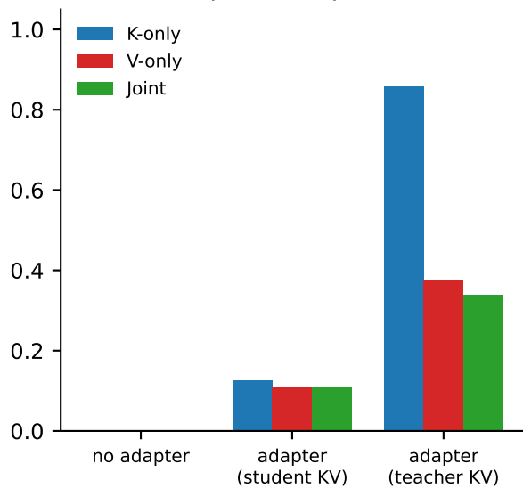
(b) Consumption adapter (8B→0.6B)
