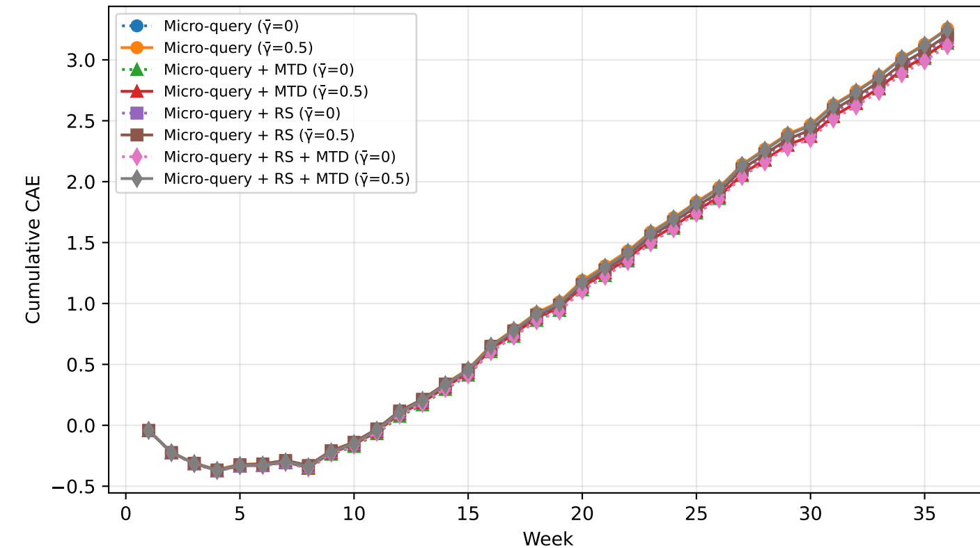
Cumulative CAE over time, aggregated
