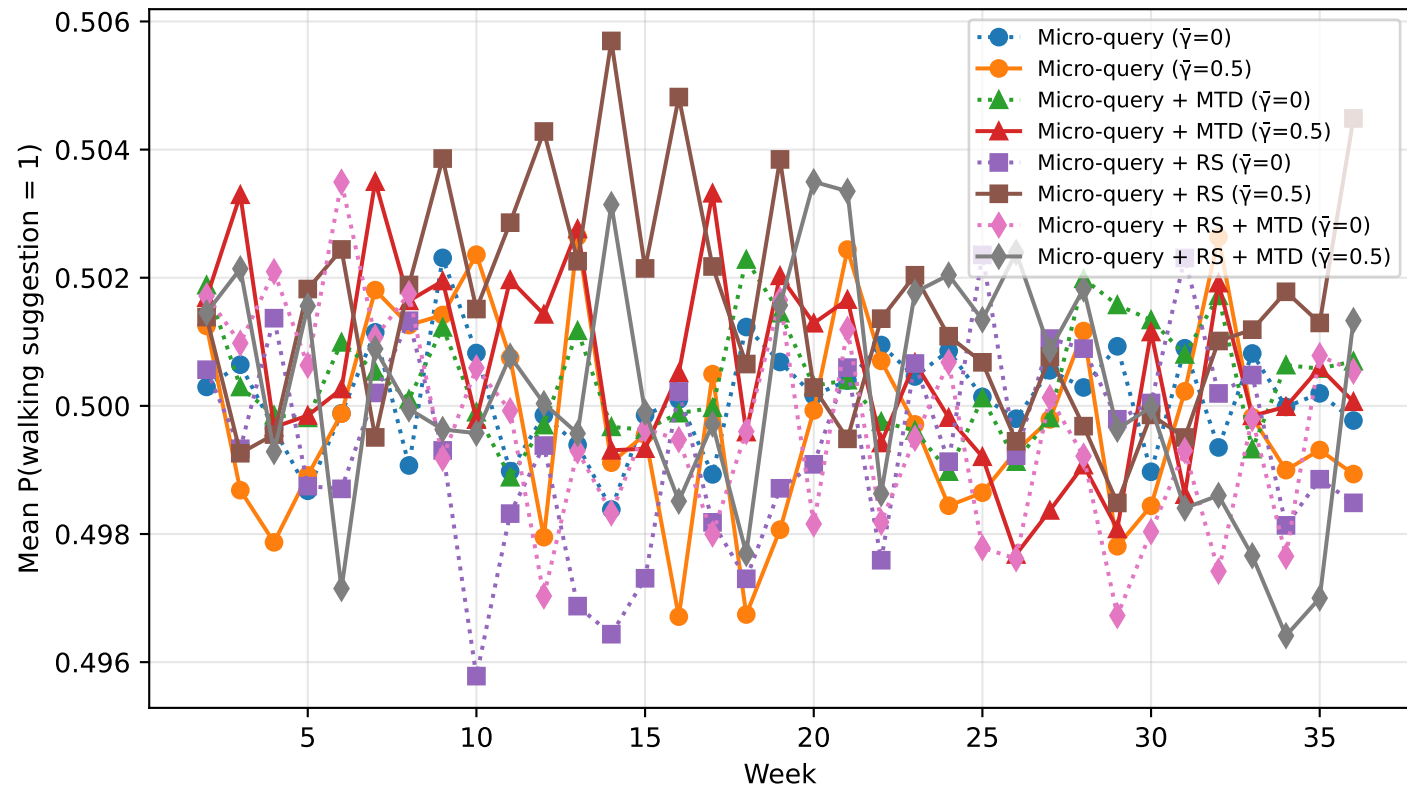
Action probability over time, aggregated
