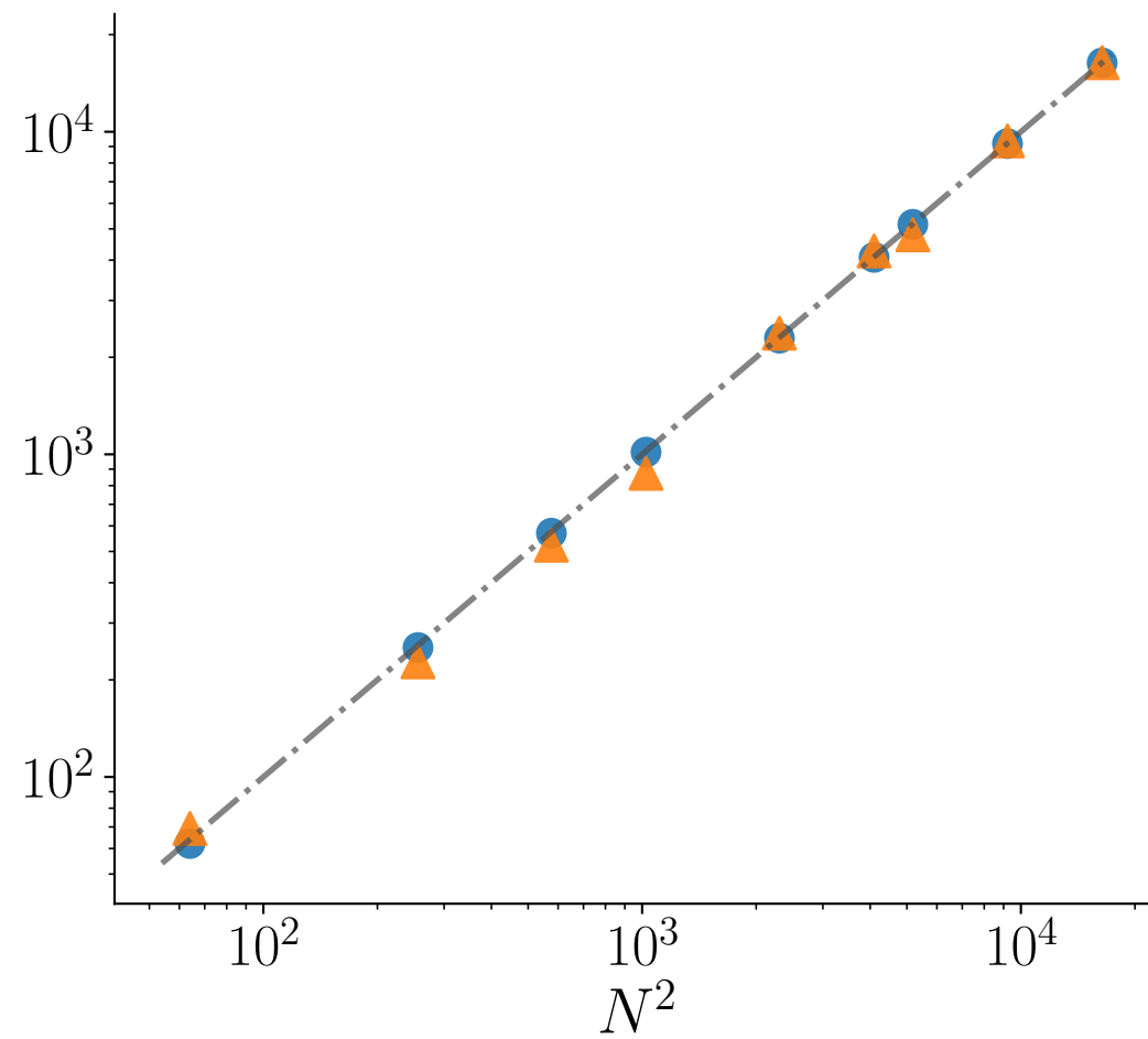
Stone-Wales
