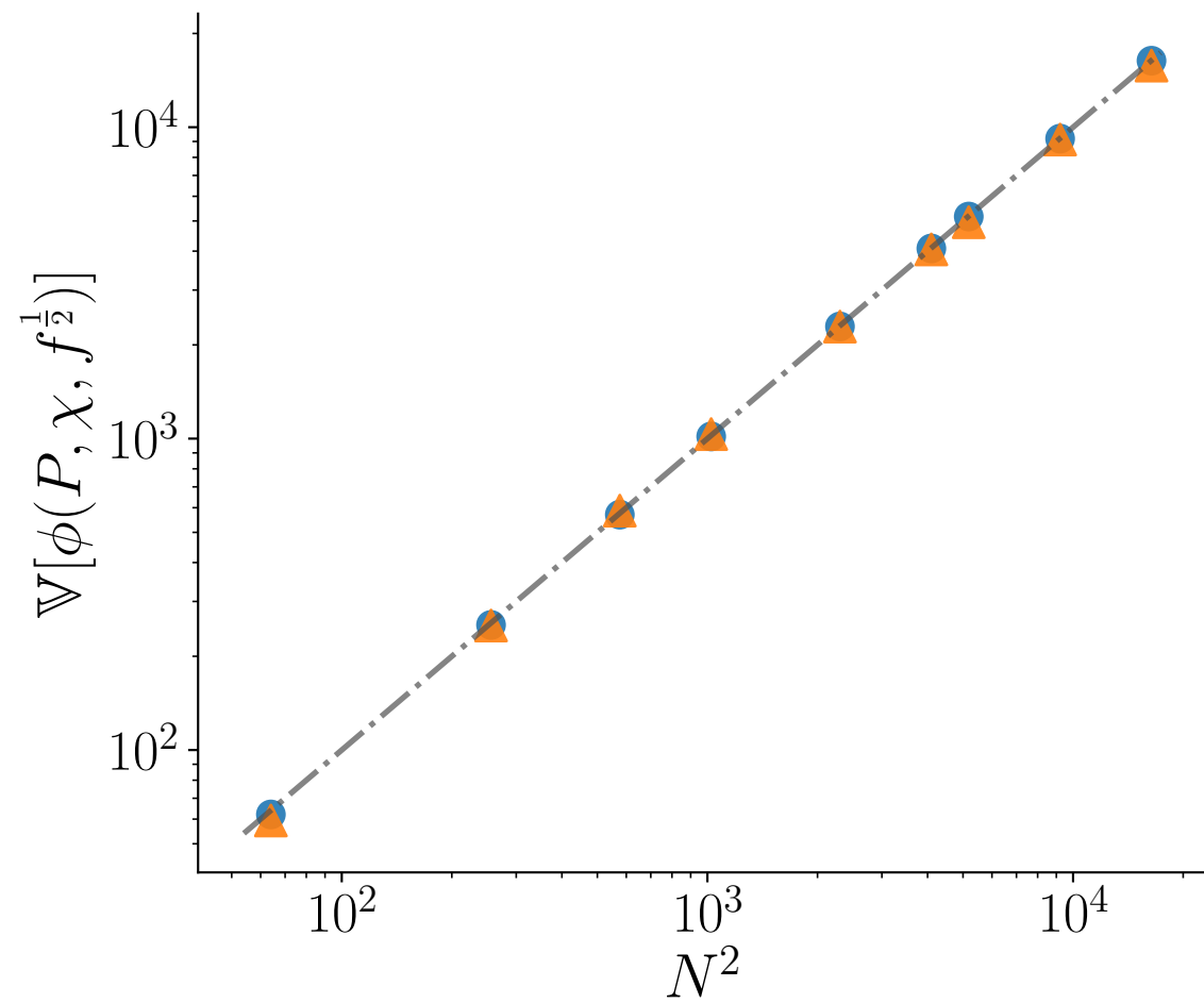
Perfect lattice
