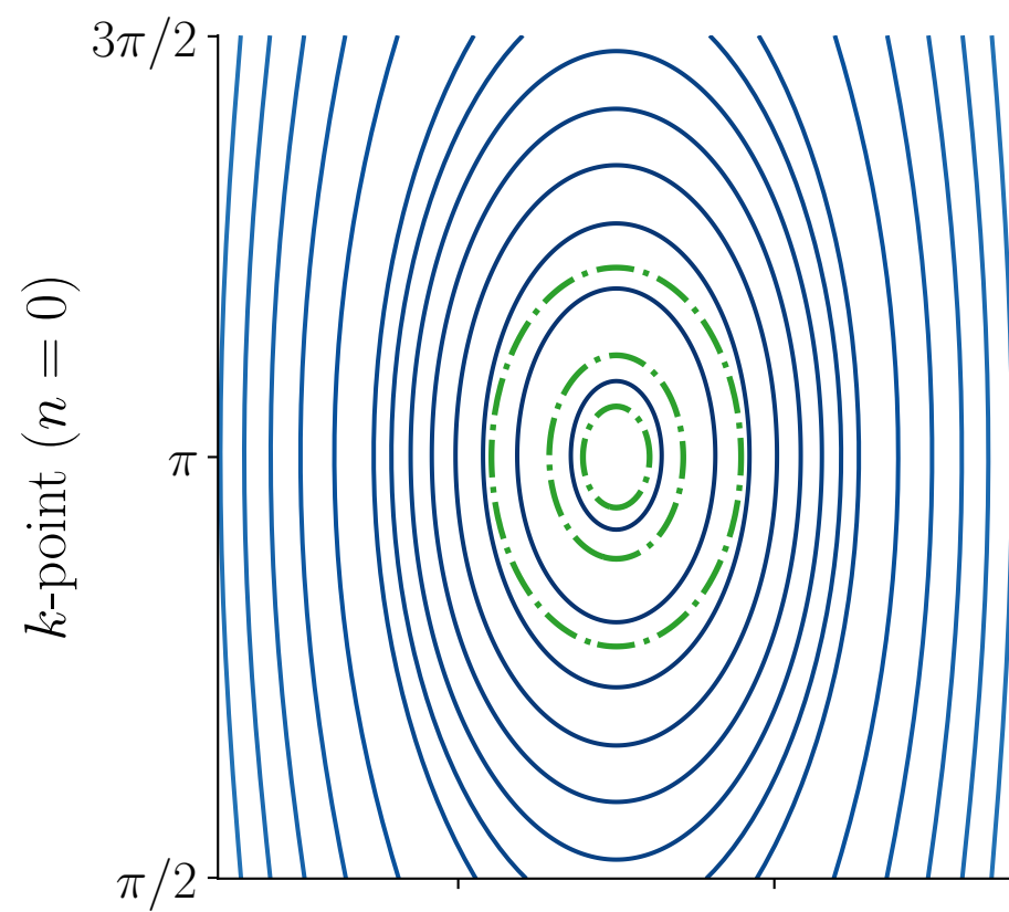
E_1(k, X) near p = 1
