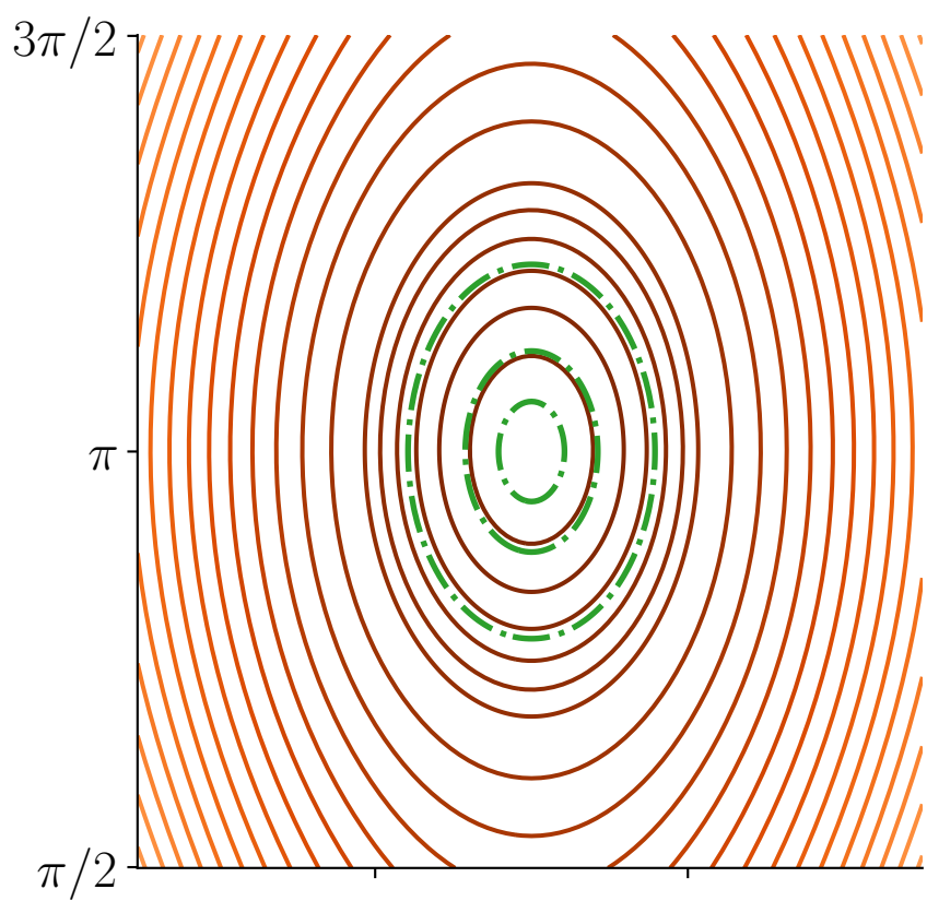
E_2(k, X) near p = 2
