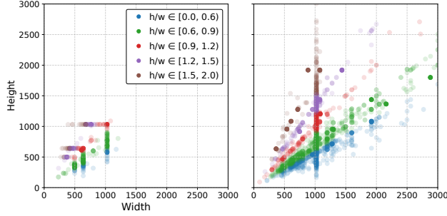
Figure 3. Resolution scatter plots of DIPA2 (left) and our dataset (right). Each point corresponds to a single image, plotted by its width and height, and colored by aspect ratio ( h/w ). Compared to DIPA2, our dataset contains substantially more samples, exhibits noticeably higher overall resolution, and spans a wider range of aspect ratios.
