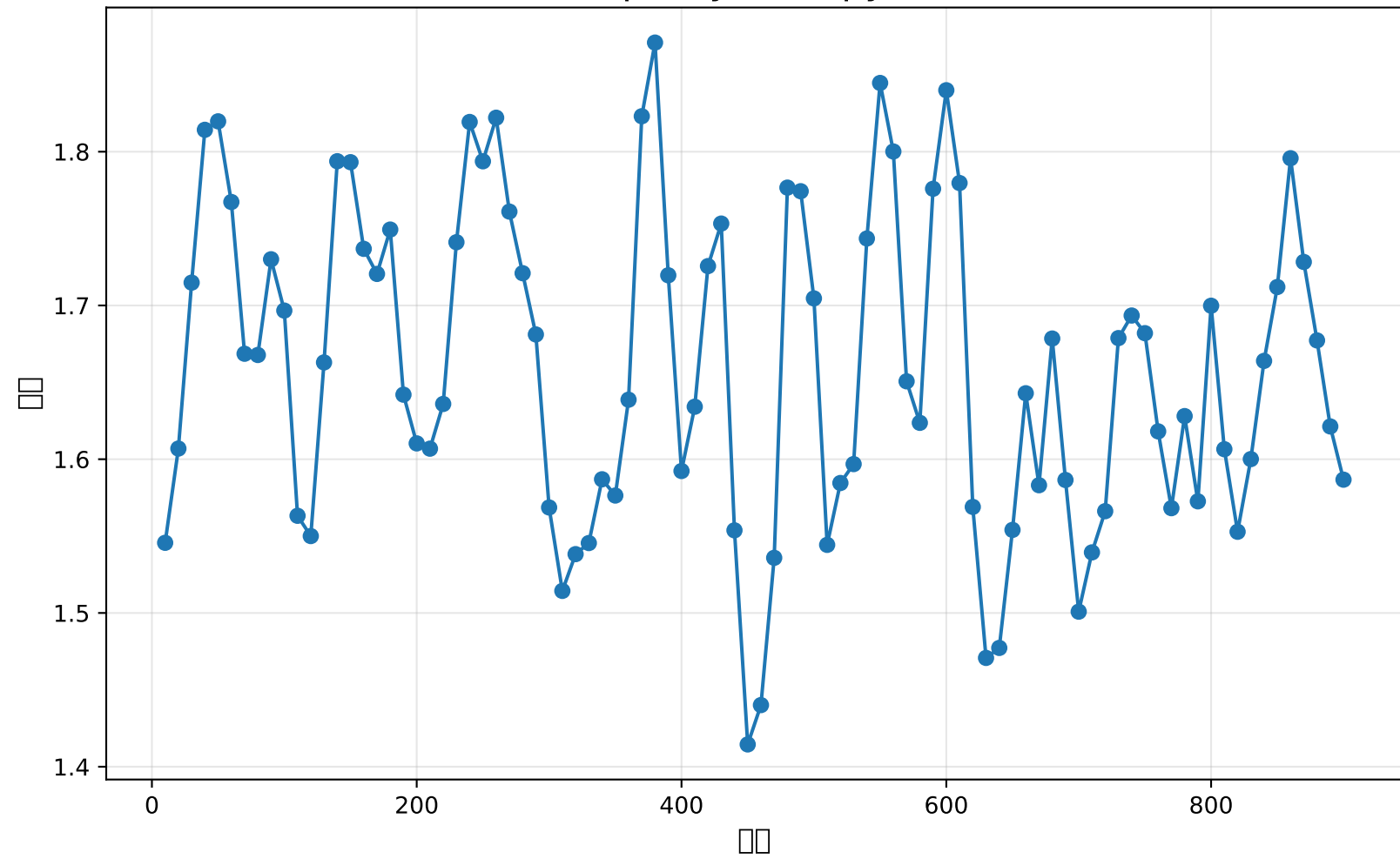
policy entropy
