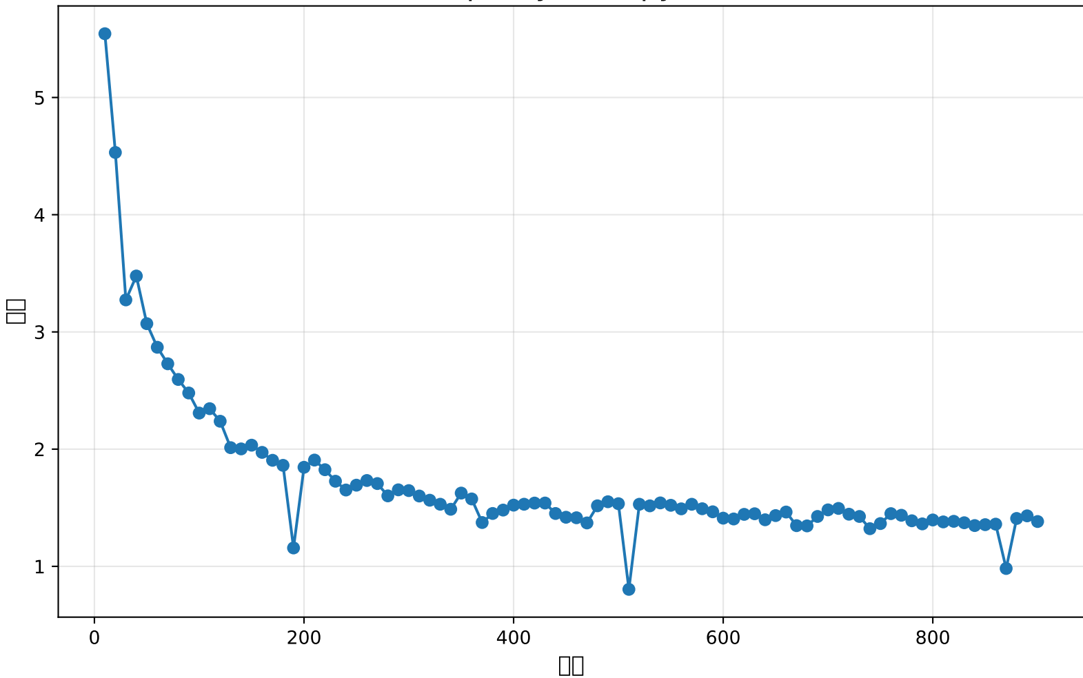
policy entropy
