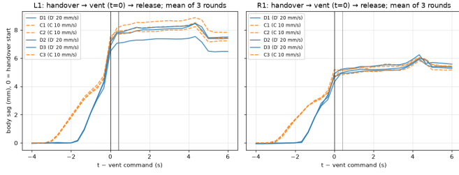
Fig. 5. The discrimination result, seen directly: handover profiles of all six runs aligned on the vent command ( t=0 ), per-leg means over rounds (left L1, right R1). At double transfer rate ( D' , solid) the descent ramp is twice as steep as the control ( C , dashed) but ends at the same plateau—the descent tracks the millimeters transferred, not elapsed time. [TODO: restyle to match the other figures (fonts/colors); currently the analysis-report rendering].
