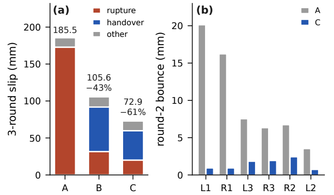
Fig. 4. Where the loss lives ( n=3 means). (a) Three-round slip by segment and condition: the handover converts an impulsive 173 mm rupture loss into a 60 mm quasi-static transfer loss; weights compress it to 40 mm. (b) Per-leg round-2 rupture bounce, A vs. C: the stiff front legs drop from 20.1/16.2 to 0.9/0.9 mm.
