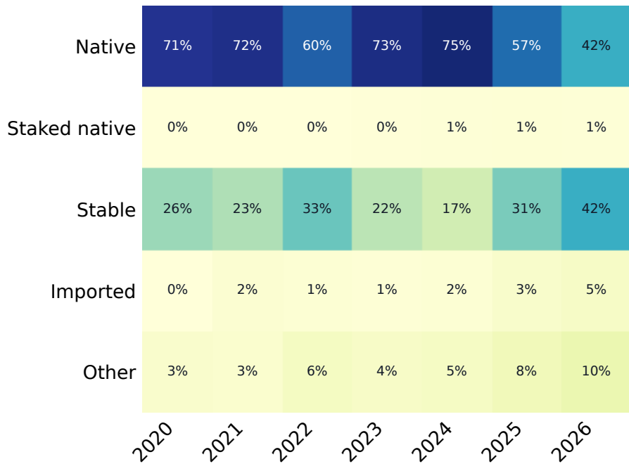
Intermediary episodes
