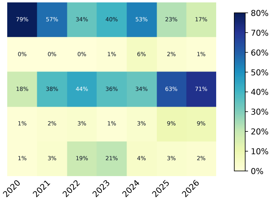
Routed value
