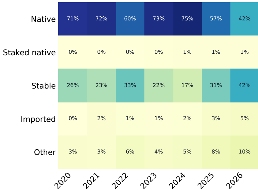
Route count
