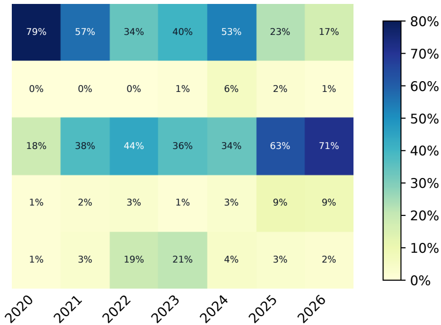
Route value
