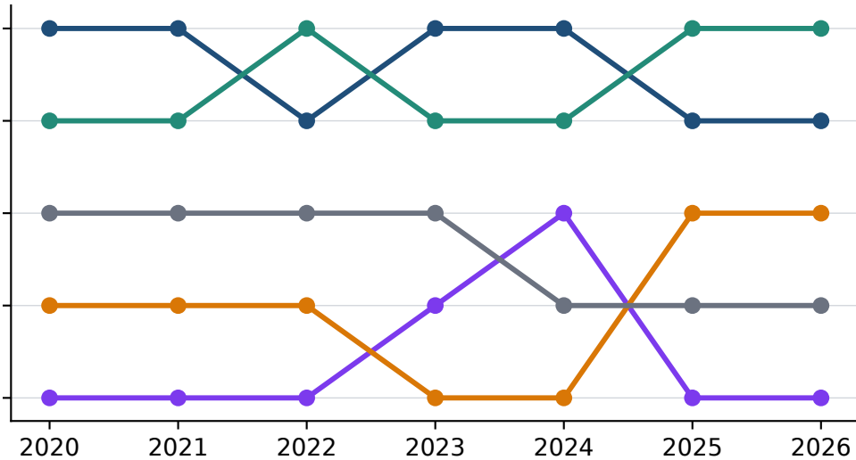
Routed value
