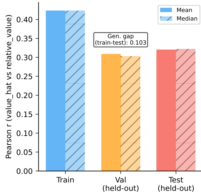
(C) Mean/Median PCC by split
