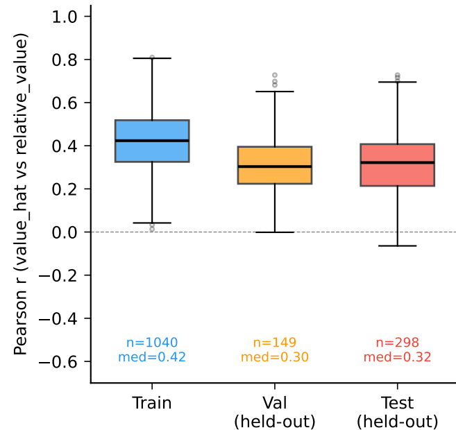
(A) PCC distribution per data split
