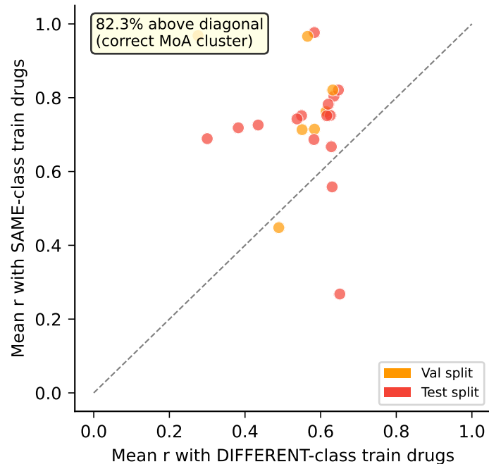
(B) Held-out drug MoA cluster recovery (test/val vs train drugs)
