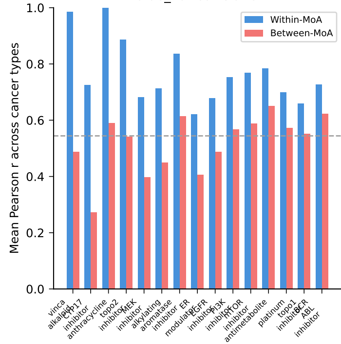
(A) Within vs between MoA value_hat correlation
