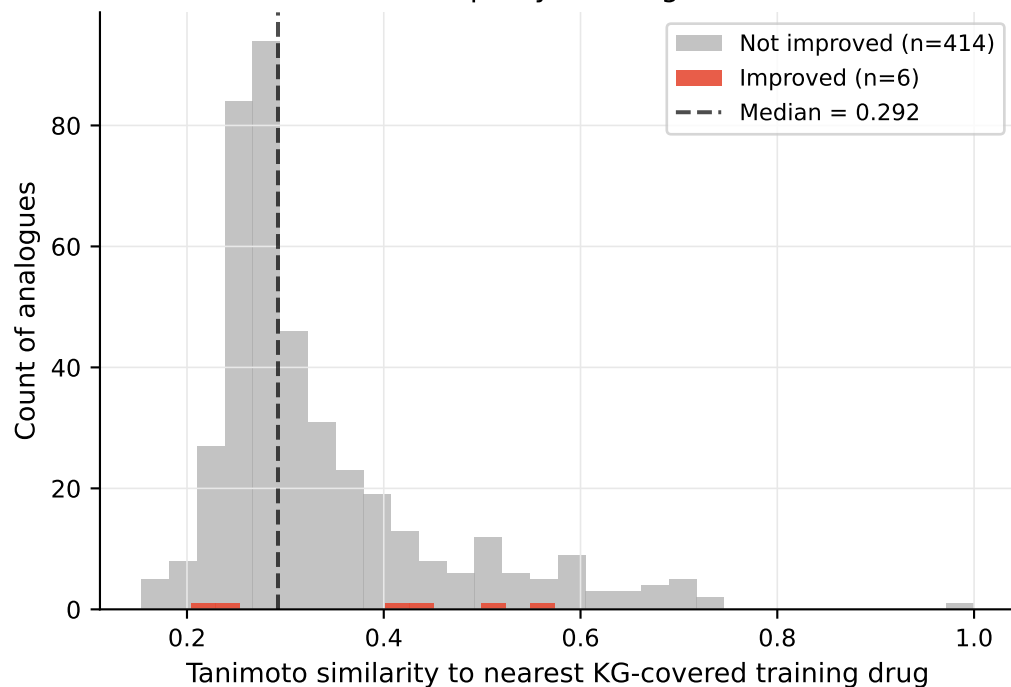
Erlotinib analogues (TCGA-LUAD) KG proxy coverage
