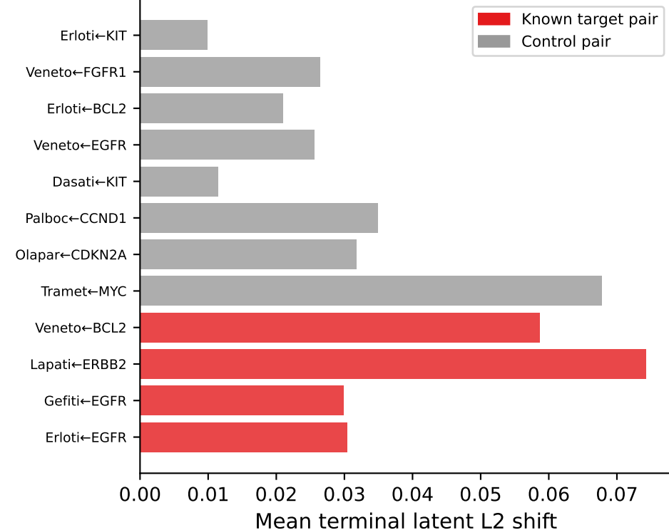
Terminal Latent Shift after Gene Silencing
