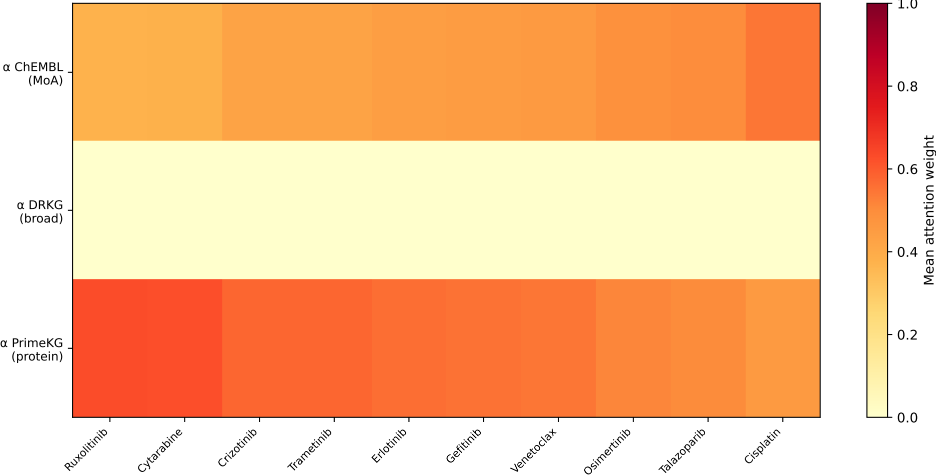
A. KG Attention Profiles for Unseen Test Drugs (World model dynamically allocates attention to three prior networks)
