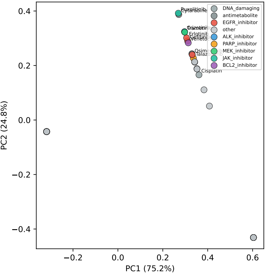
B. Drug KG Attention Clustering (Same-family drugs cluster → mechanism learned from KG)
