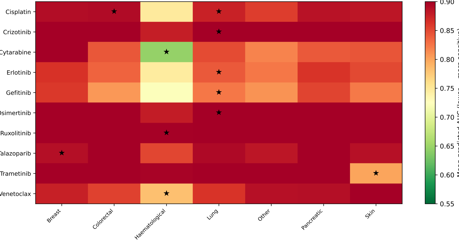
C. KG-Predicted Cancer Type Sensitivity Map ★ = Known clinical indication (validation)
