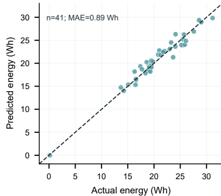
Held-out telemetry fit
