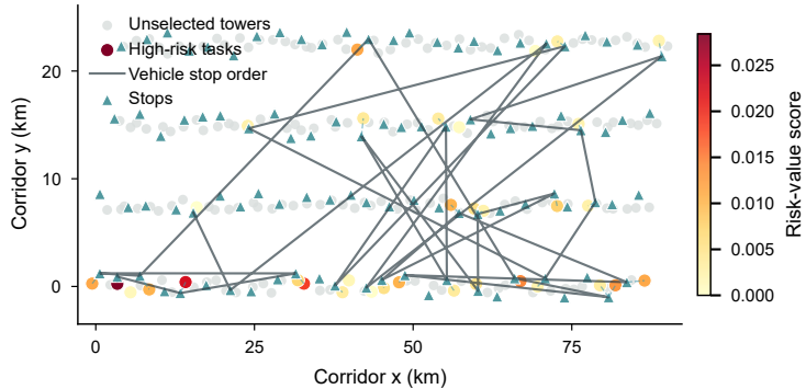
Solved dispatch network
