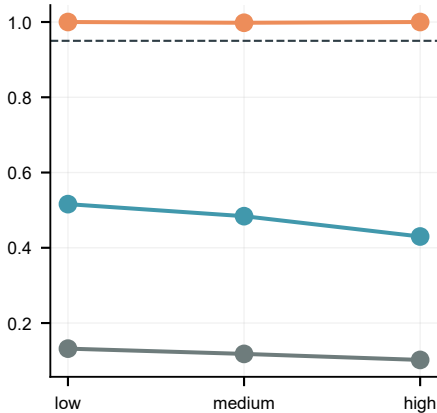
95% coverage
