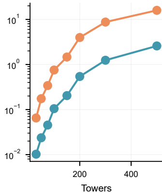
Runtime
