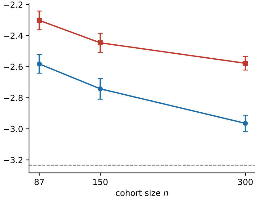
time slope \beta_{\text{time}}
