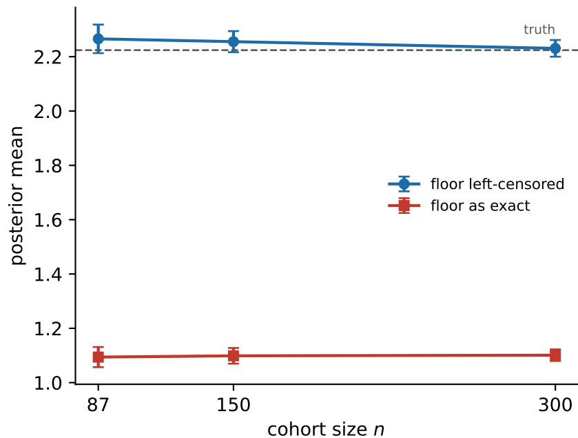
random-slope SD \tau_{b1}
