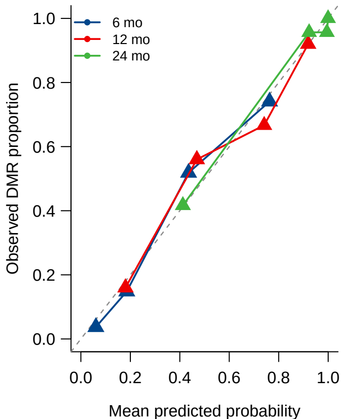
Recalibrated
