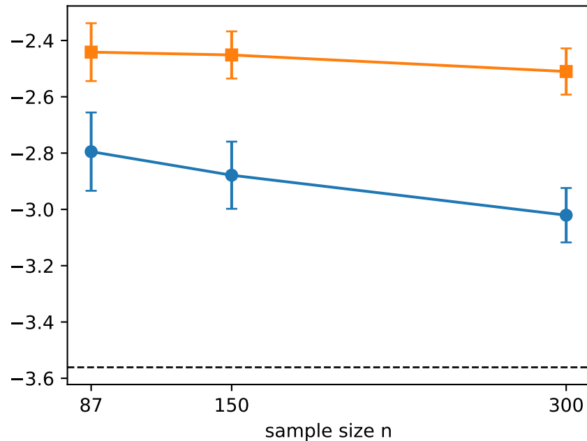
Time slope \beta_{time}
