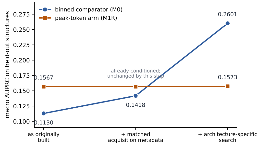
Corrections to the comparator
