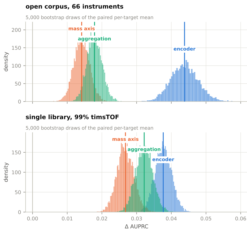
Figure S1: Bootstrap distributions of the three effects on each corpus. On the open corpus the encoder distribution is separated from the other two; on the single-library corpus all three overlap, and the mass-axis and aggregation distributions overlap heavily — which is the same fact Table S3 records as a sign reversal.
