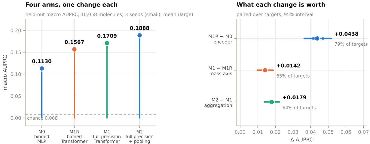
Figure 1: Decomposing the gain on the open corpus. Left: held-out macro AUPRC for the four arms; small dots are individual seeds, large dots their mean. Right: what each single change is worth, paired over targets with 95% bootstrap intervals; small dots are the per-seed effect sizes.
