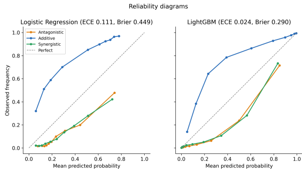
Figure 4: Reliability diagrams for both models, with expected calibration error and multiclass Brier score in each panel title. LightGBM (right) is substantially better calibrated than the logistic baseline (left); in both models the re-weighted rare classes lie below the diagonal, indicating over-confidence.
