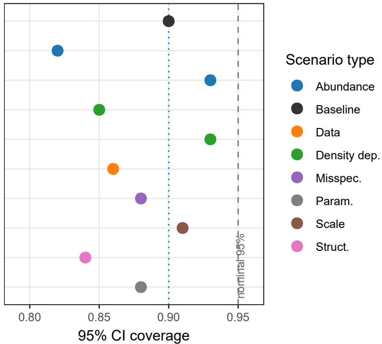
(b) Uncertainty quantification
