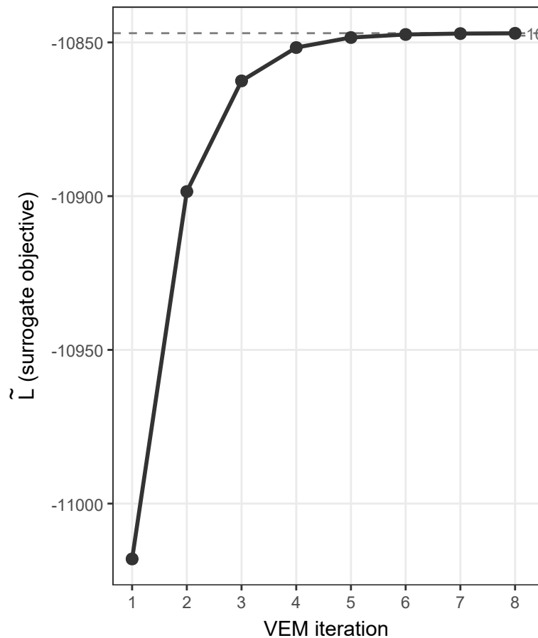
(b) ELBO convergence
