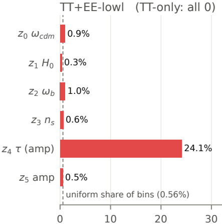
(a) on-manifold gradient mass at \ell < 30 (EE) [%]
