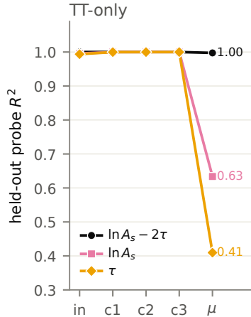
(b) linear decodability: input \rightarrow conv blocks \rightarrow posterior mean
