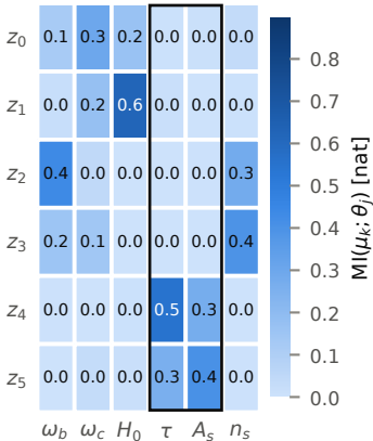
TT+EE-lowl
