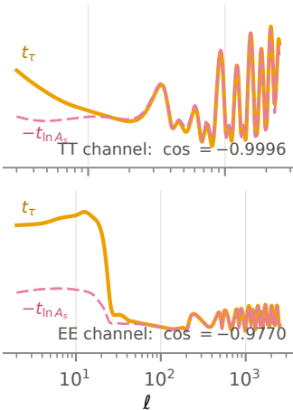
(a) templates in design space ( -t_{\ln A_s} flipped)
