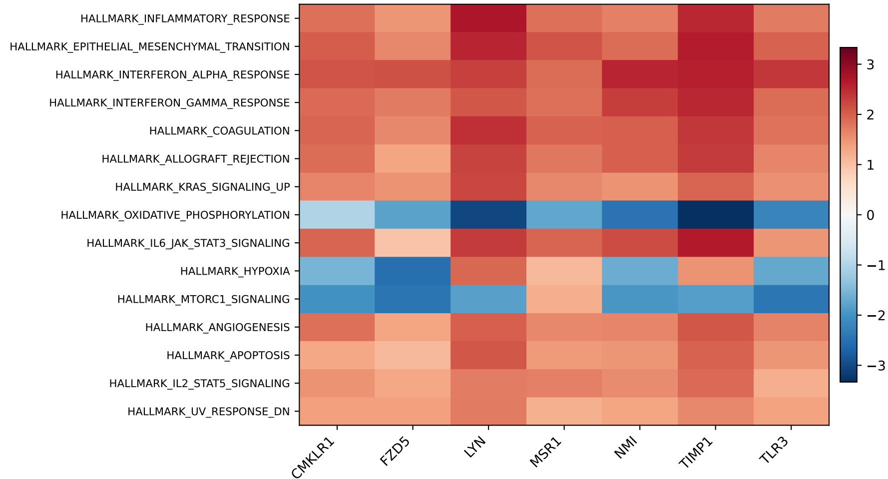
Gene-specific preranked GSEA NES
