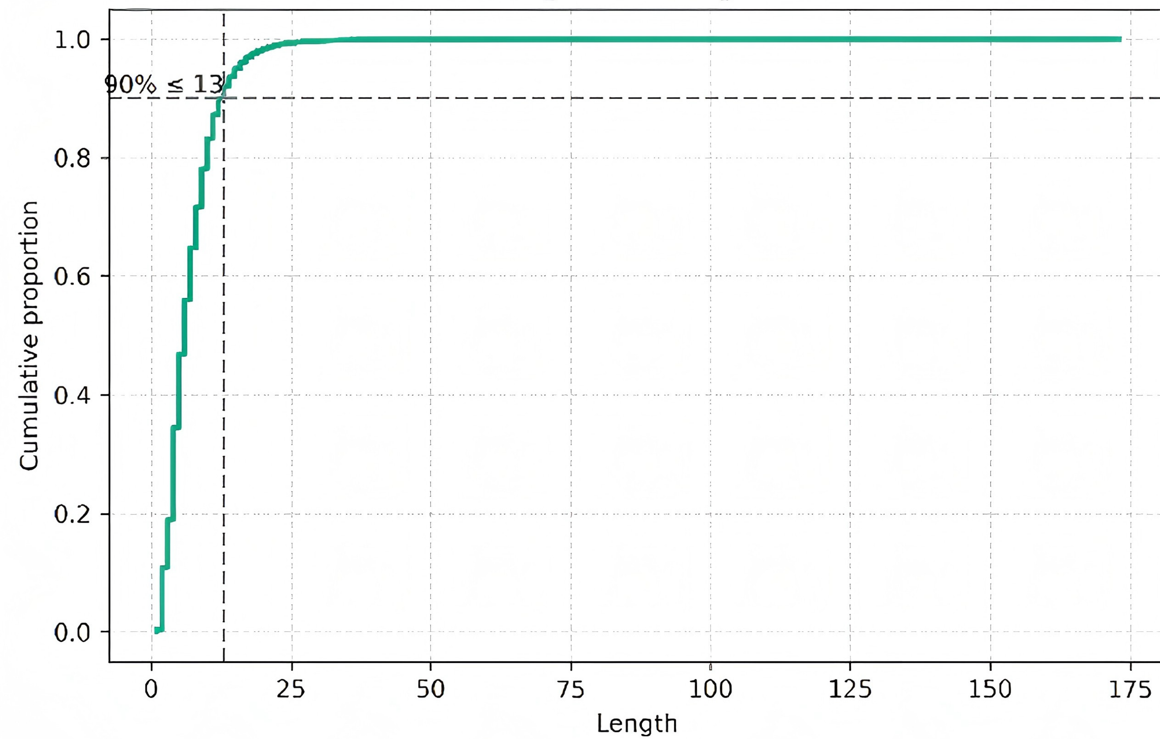
Argument Length
