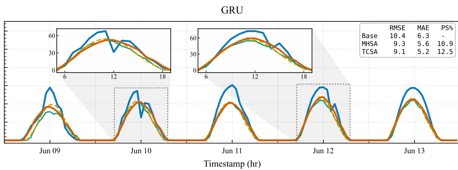
(b) Solar Plant - II
