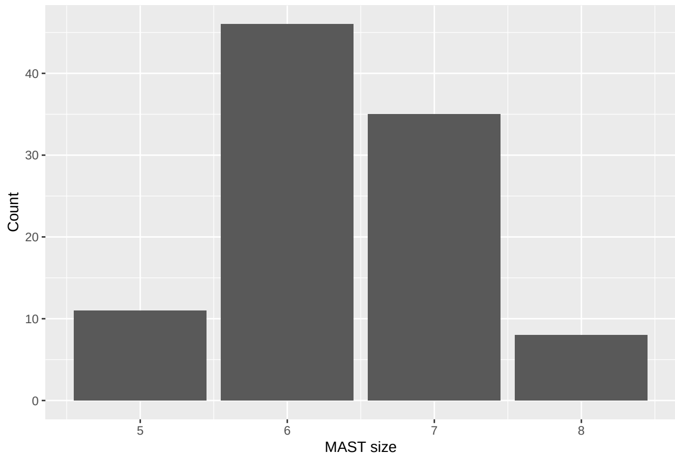
Radish bootstrap MAST vs reference
