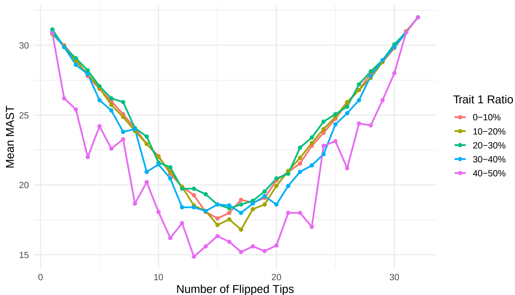
Simulation 2: Mean MAST under increasing tip flipping
