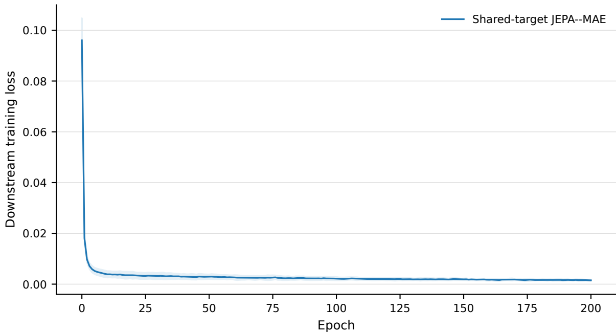
Downstream training loss (mean across stocks after seed averaging)
