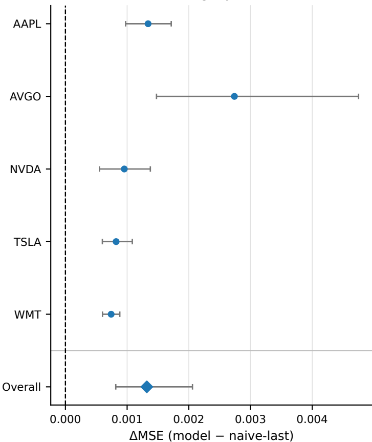
Shared-target JEPA--MAE
