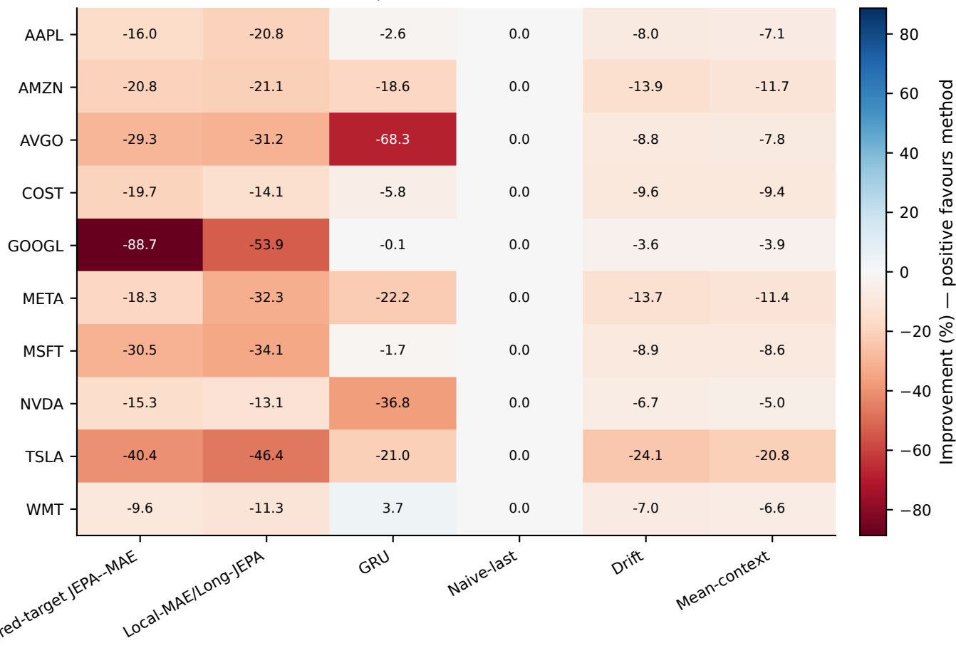
Relative MSE performance versus naive-last
