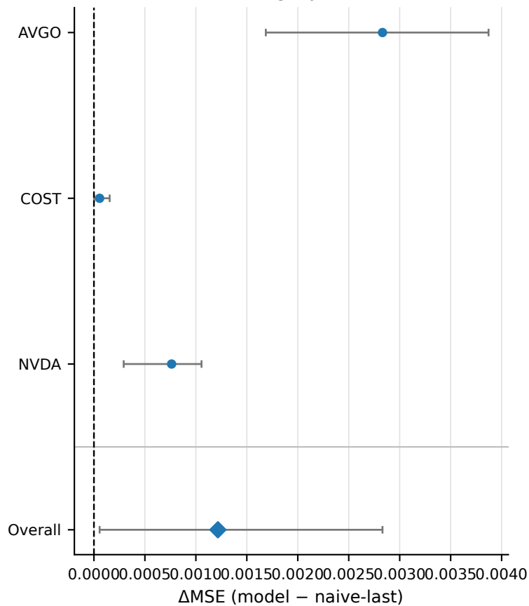
Shared-target JEPa--MAE
