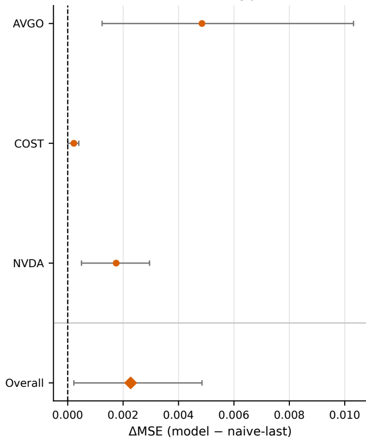
Local-MAE/Long-JEPa
